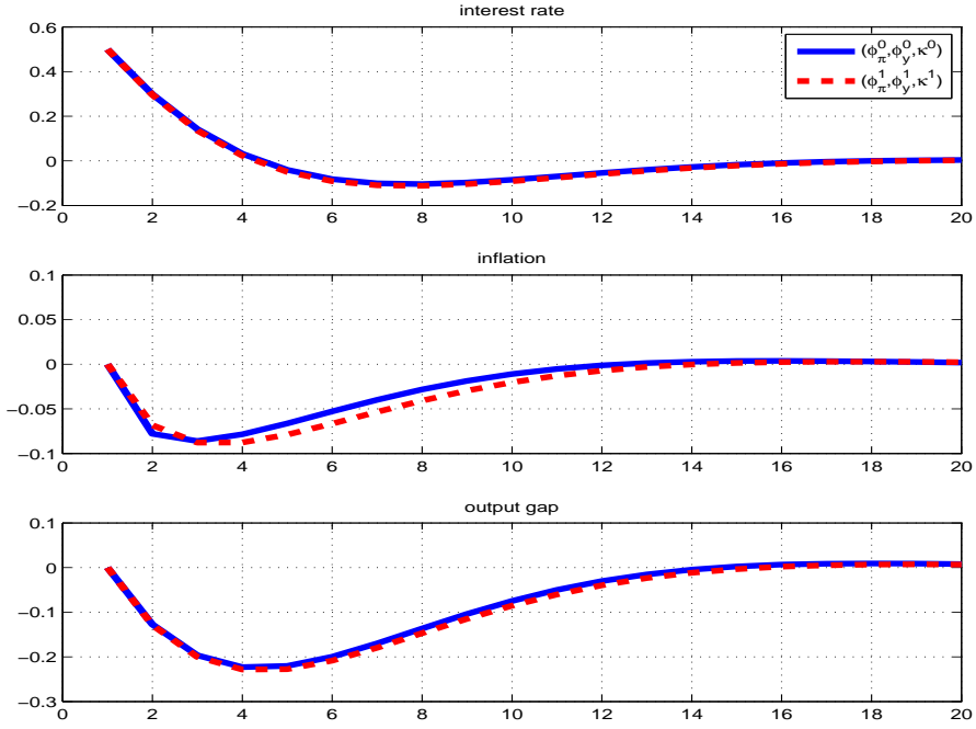
Figure 6 - VAR on simulated data
