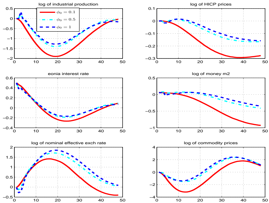
Figure 5 - Robustness check on the prior tightness - sample 1999-2007
