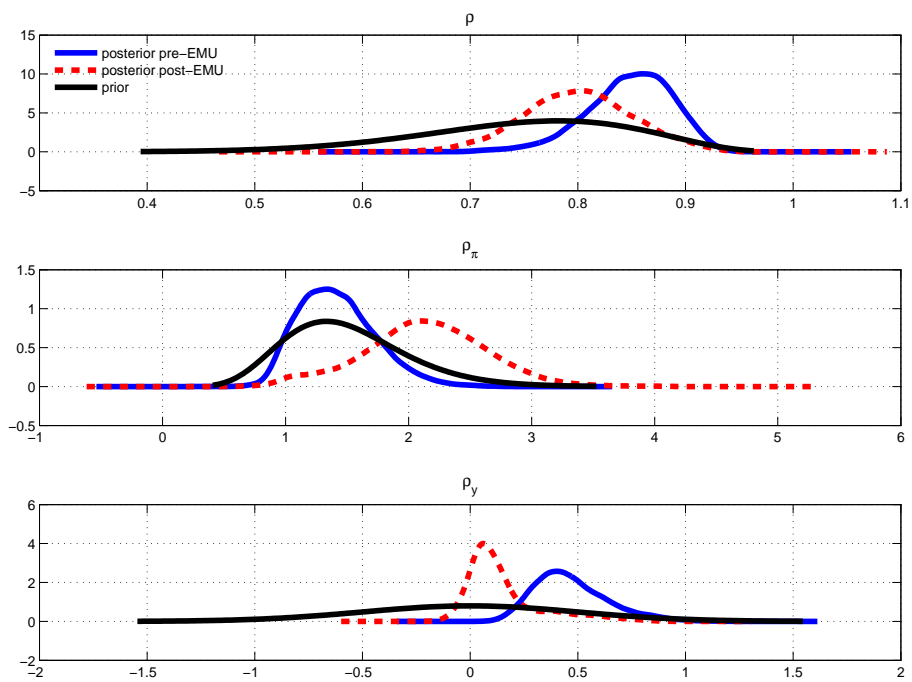
Figure 8 - Prior and posterior marginal distributions: monetary policy rule
