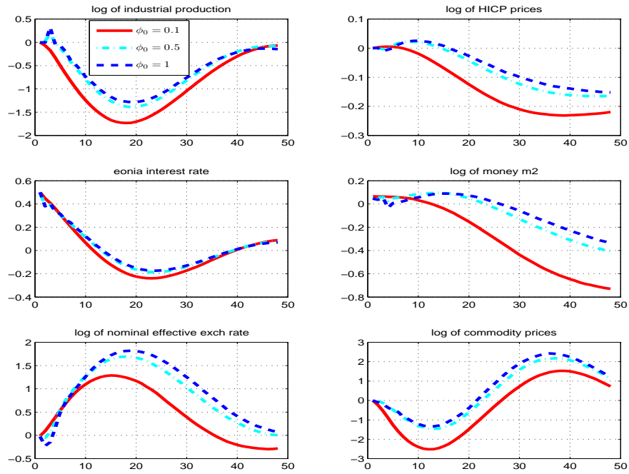
Figure 4 - Robustness check on the prior tightness - sample 1994-1998
