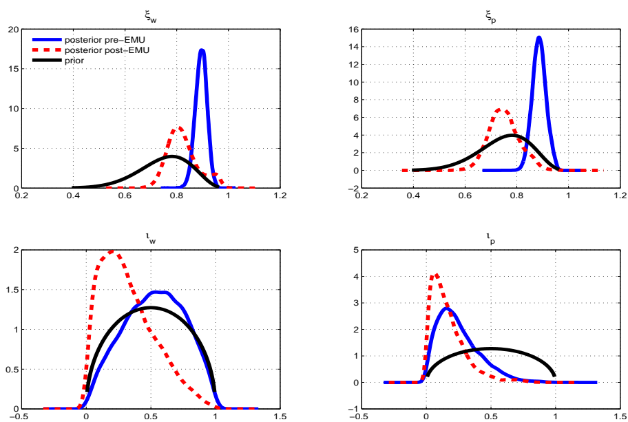
Figure 7 - Prior and posterior marginal distributions: nominal rigidities
