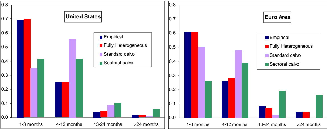
Figure 2: Empirical and model based distributions of price durations
