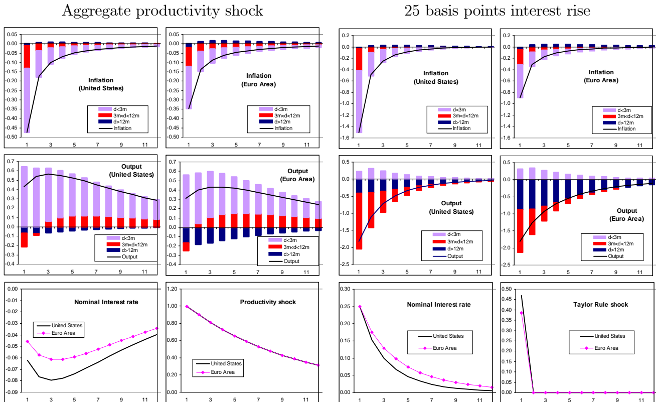
Figure 4: Impulse response functions to aggregate shocks.
