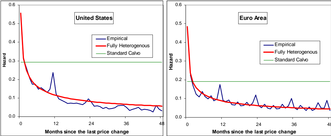
Figure 3: Empirical versus fitted hazard
